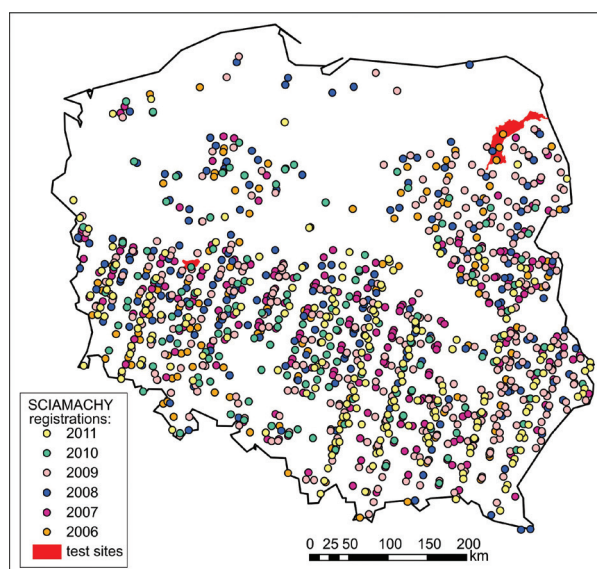
Fig. 1. Spatial distribution of SCIAMACHY \text{XCO}_2 measurements for Poland for the years 2006 to 2011
