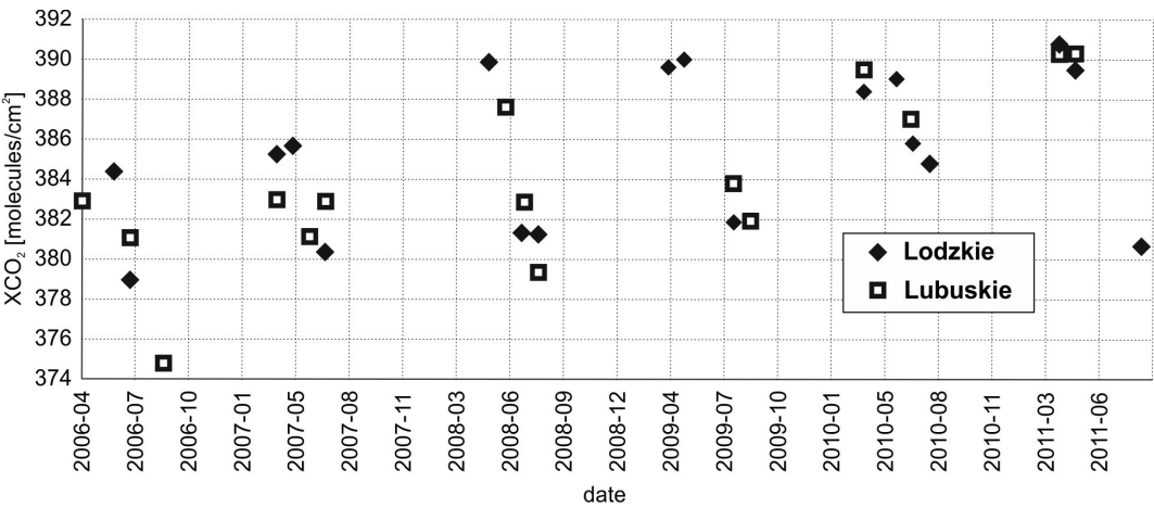
Fig. 7. Monthly variability of XCO 2 values in Lodzkie and Lubuskie Voivodeships
