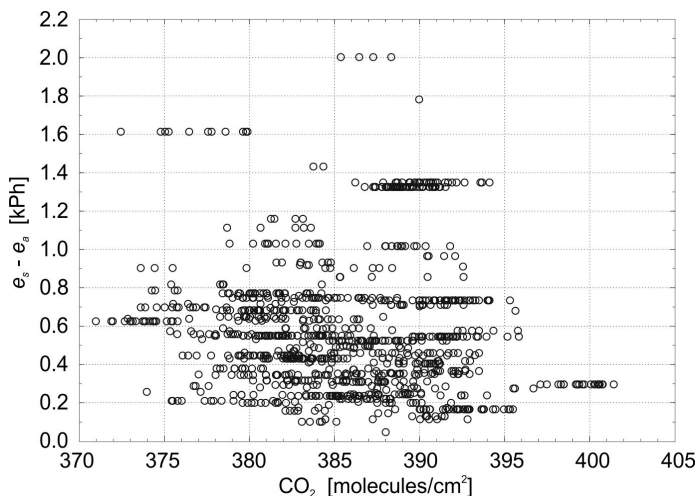
Fig. 6. Relationship between daily SCIAMACHY registration of \text{CO}_2 and computed water pressure deficit for Poland
