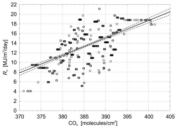
Fig. 5. Relationship between daily SCIAMACHY registration of \text{CO}_2 and computed daily net radiation R_n for Poland
