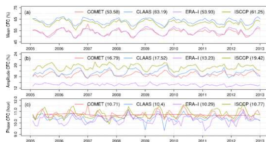
Figure 4: Time series of mean, amplitude and phase of CFC diurnal cycle from COMET, CLAAS, ISCCP and ERA-Interim aggregated from all grids within Meteosat disc. Values in brackets represents the mean over the 2005-2013 period.
