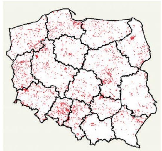
Fig. 4. Land use changes in Poland in a period 1990–2000
