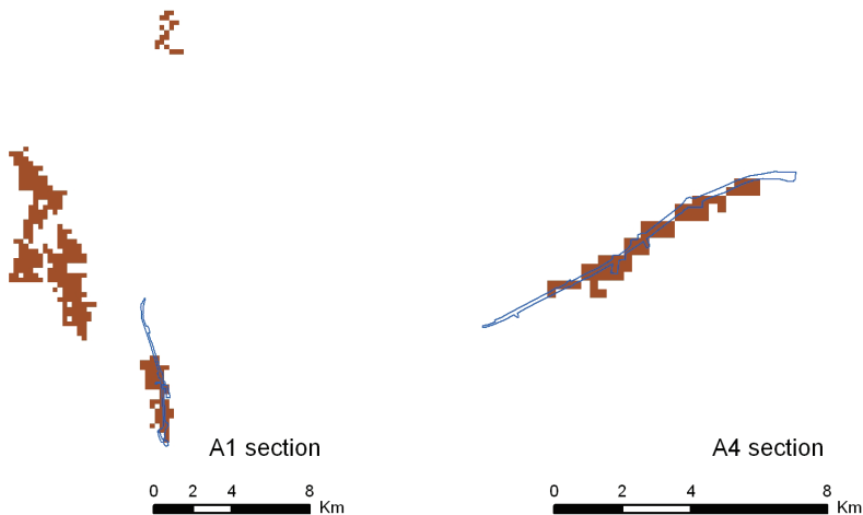
Fig. 6. Brown colour – the final result of changes. Blue colour – reference layer changes from CLC 2000–2006
